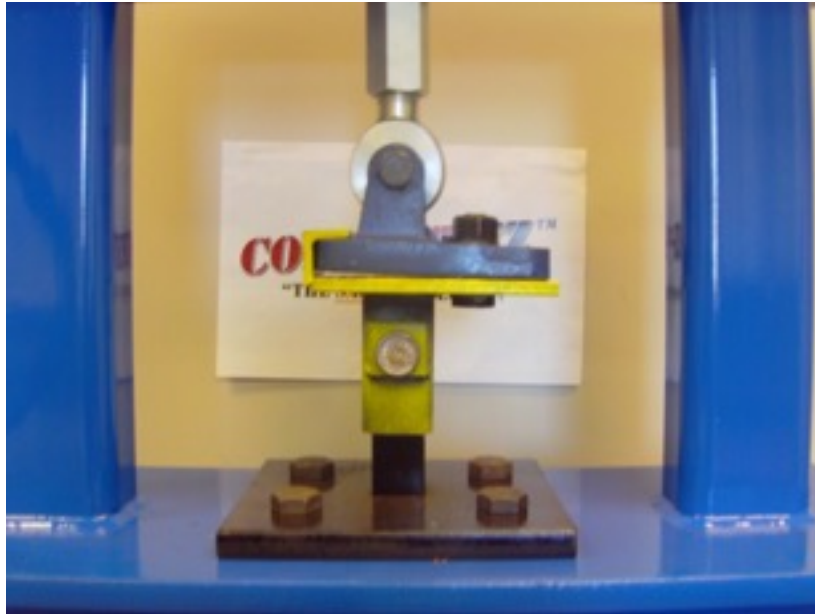
Figure 3: Dayton Superior 12 K Shoe; 0.375 Plate, 0.25 Angle;
